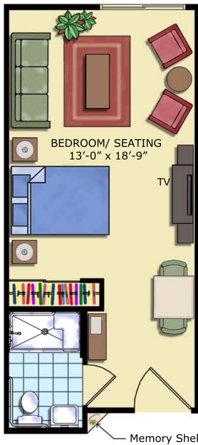
PRIVATE SUITE 368 s.f. (13'-0" x 29'-0")
